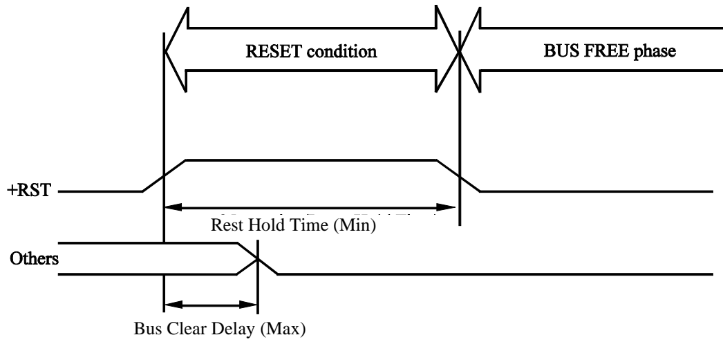
Figure 7.20 RESET condition
