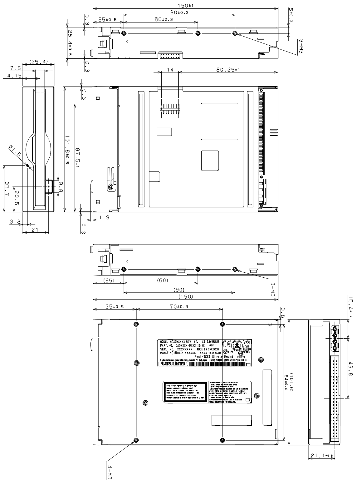
Figure 3.2 Outer dimensions (1 of 2)
