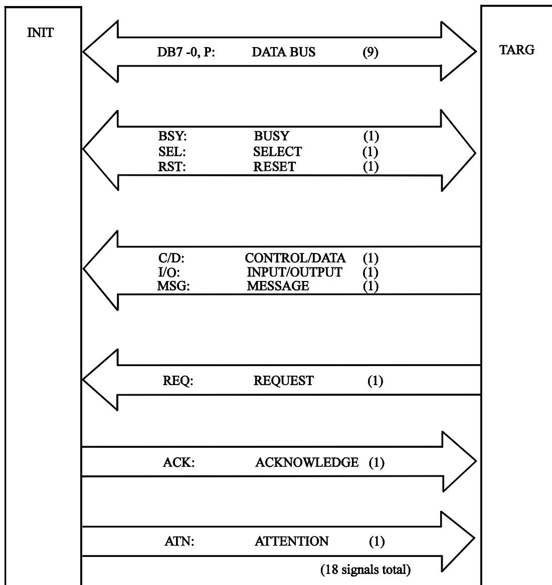
Figure 7.2 Interface signals
