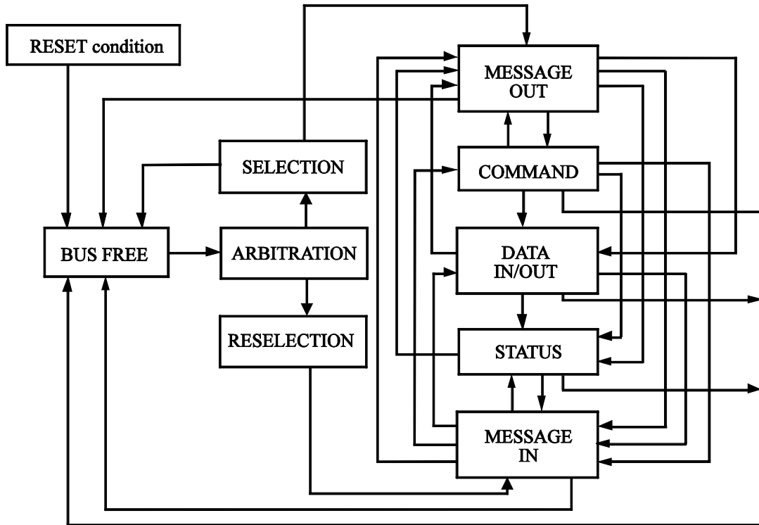
When ARBITRATION is used without MESSAGE OUT
