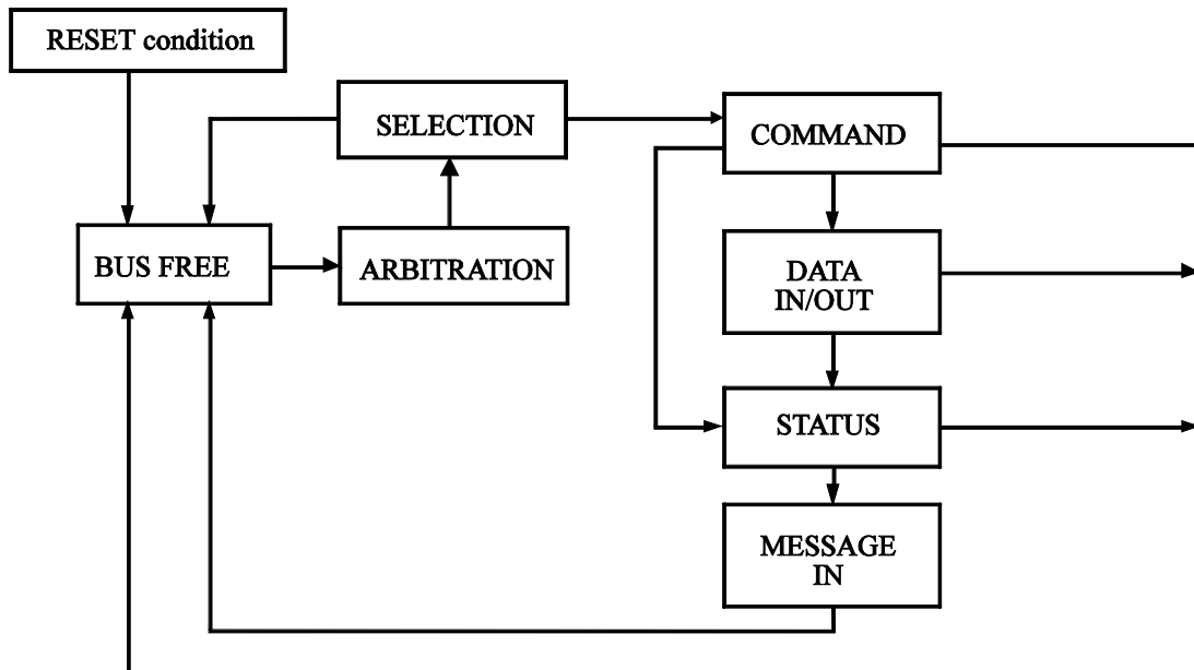
Figure 7.21 Bus phase sequence (1 of 2)
